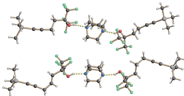
Figure 3. X-ray crystal structures of the DABCO adducts of the fluorinated alkynol 4a (top) and 4b (bottom). Dark gray C, white H, blue N, red O, green F, light gray Si.
