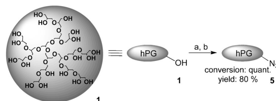
Scheme 2. Modification of the functional groups of dendritic polyglycerol. Reagents and conditions: a) \text{MsCl} , pyridine, 0^\circ\text{C} , 16 h; b) \text{NaN}_3 , DMF, 100^\circ\text{C} , 16 h. Ms = methanesulfonyl.
