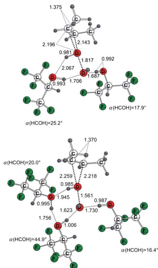
Figure 1. Catalysis of (Z)-2-butene epoxidation, effected by two (top) and three (bottom) molecules of HFIP, through hydrogen-bonding networks (from Ref. [3b]).
