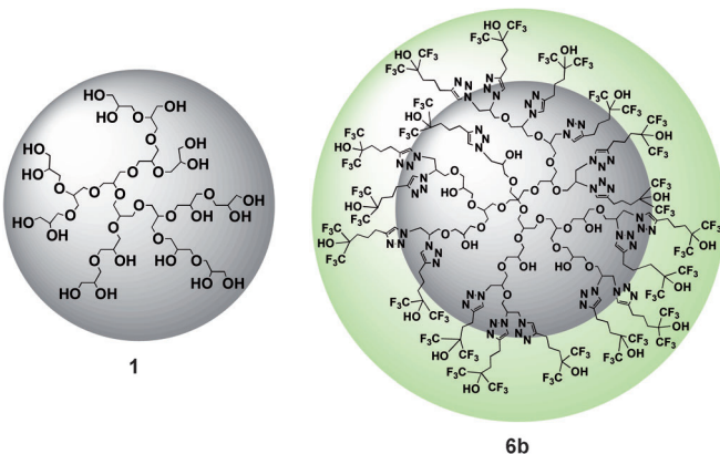
Figure 2. Epoxidation catalyst 6b based on hyperbranched polyglycerol 1 as a polymeric support for HFIP analogues.
